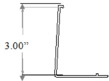
3.00" square fascia
