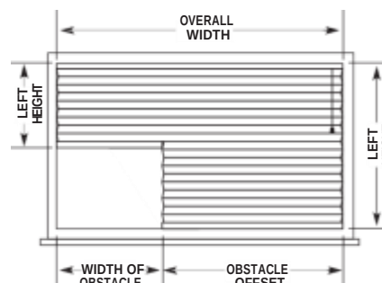
2-on-1 Headrail
